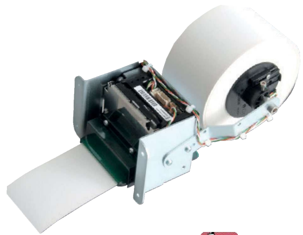
Auto cutter
